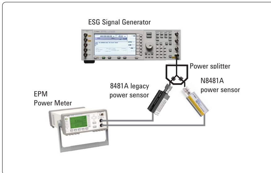
Figure 7. EPM, 8481A, N8481A, and ESG configuration diagram
