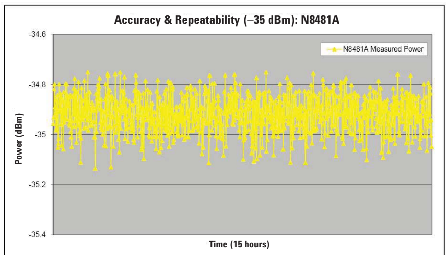
Figure 11. Measurement accuracy and repeatability graph for N8481A at power level -35 dBm.
