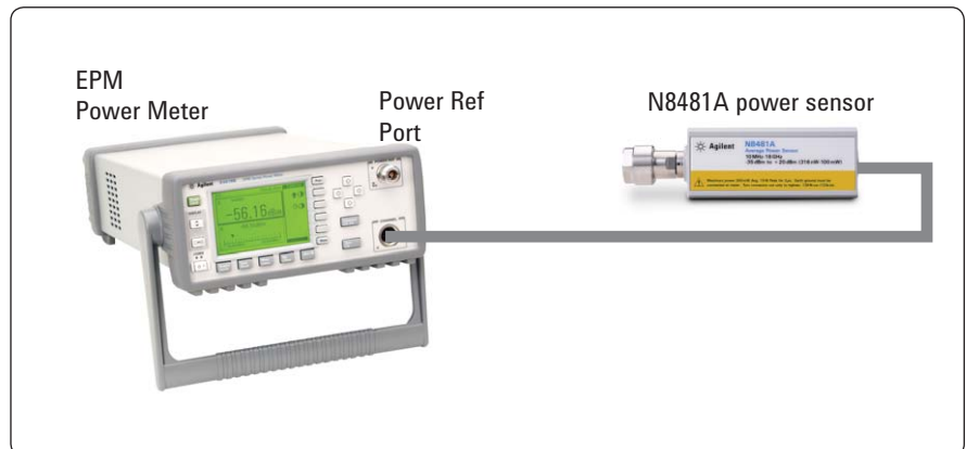
Figure 12. N8481A power sensor and EPM power meter connection configuration
