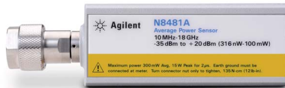
Figure 1. N8480 Series power sensor
