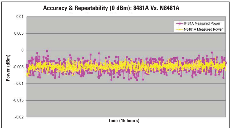
Figure 9. Measurement accuracy and repeatability graph, 8481A vs. N8481A at power level 0 dBm.
