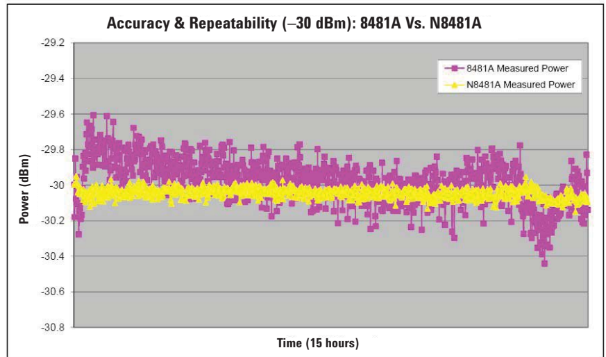
Figure 10. Measurement accuracy and repeatability graph, 8481A vs. N8481A at power level -30 dBm.
