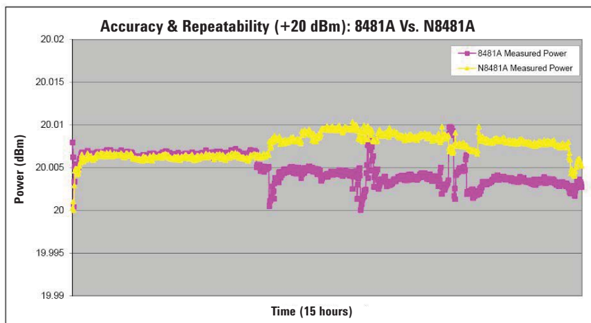
Figure 8. Measurement accuracy and repeatability graph, 8481A vs. N8481A at power level +20 dBm.
