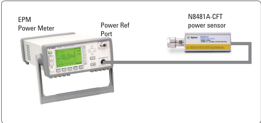
Figure 15. N8481A-CFT power sensor and EPM power meter connection configuration
