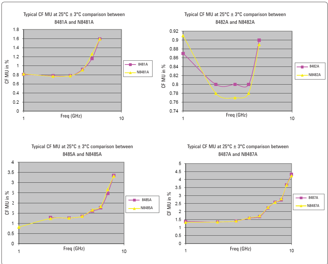
Figure 4. Typical calibration factor uncertainties comparison between legacy 8480 and N8480
